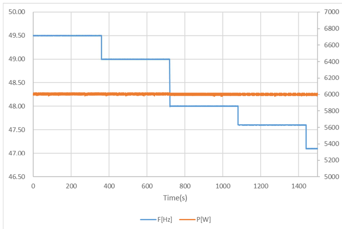
Graph of frequency a) to b) to c) to d) to e): HYD 6000-EP
